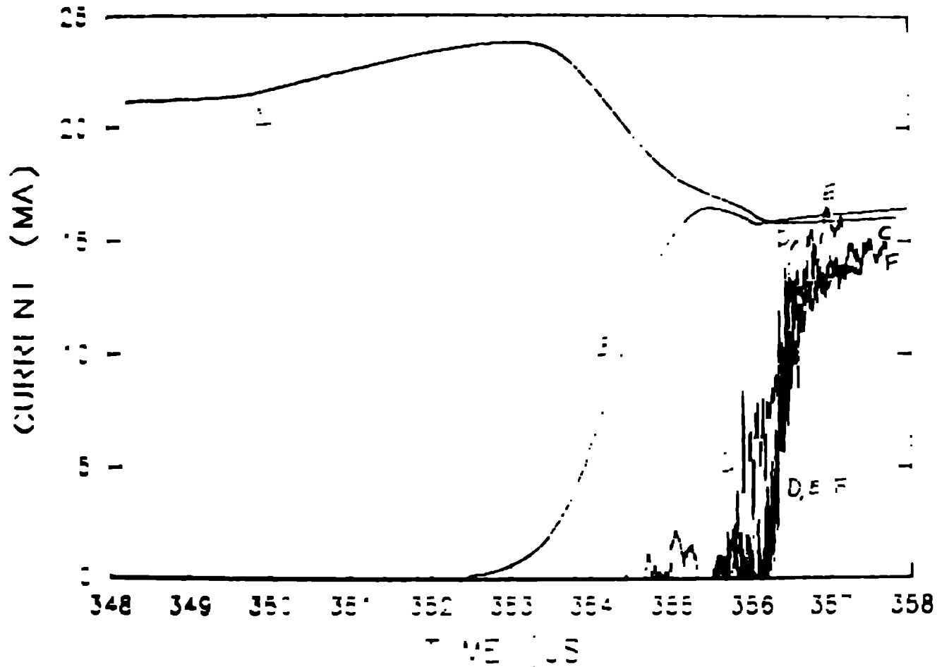
Fig 19 Selected current signals from T3. A- Storage inductor current B- Typical Faraday sensor signal showing PFS current C- dB dt sensor (integrated) 5.8 cm from graded foil on inside electrode D- Most optimistic interpretation of Faraday sensor in load slot bottom E- dB dt sensor (integrated) recessed inside load slot on upstream side. F- dB dt sensor (integrated) in bottom of load slot.
