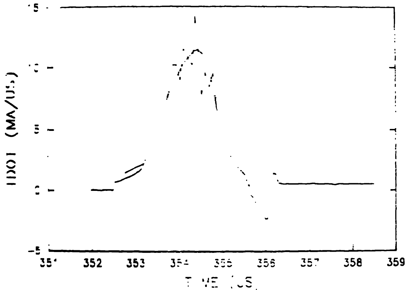
Fig. 15 \partial(I_{PF5})/\partial t combined from Rogowski coil and Faraday rotation sensors. A crude smoothing is drawn through the jagged peak area, and we estimate a peak of 11.5 MA/μs.
