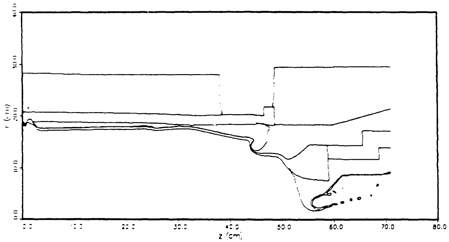
Fig 5 2-D hydrodynamic calculation of late time MK-IX output configuration.
