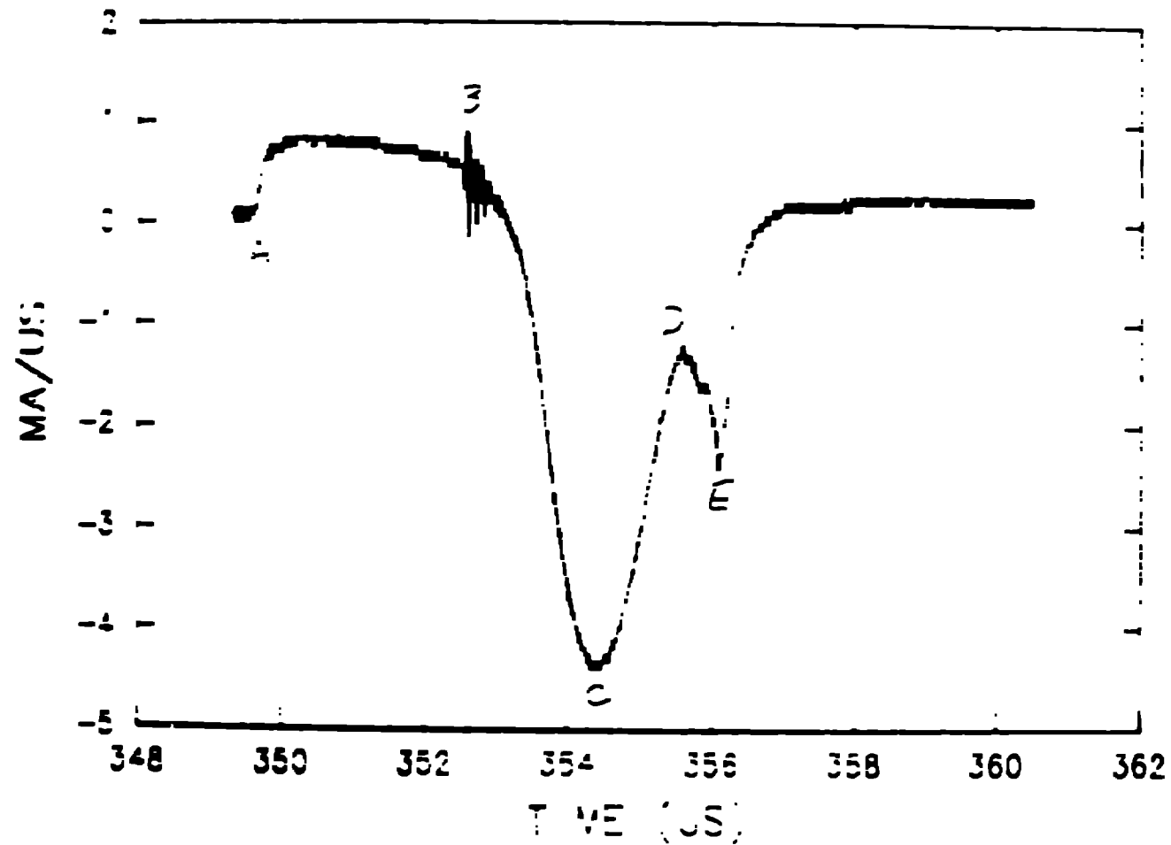
Fig 14 d(I_{STO})/dt with positions of various events marked. A- first motion of EFF conductor B- closing of detonator actuated switches C- Peak transfer rate to PFS. D- Onset of flux transfer into load slot E. Peak transfer rate into load slot.
